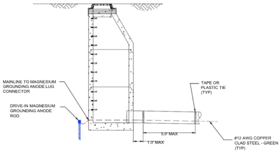
SEWER MANHOLE - SECTION VIEW NO SCALE
