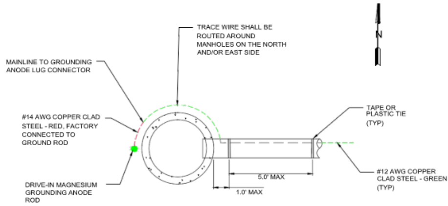
SEWER MANHOLE - PLAN VIEW NO SCALE
